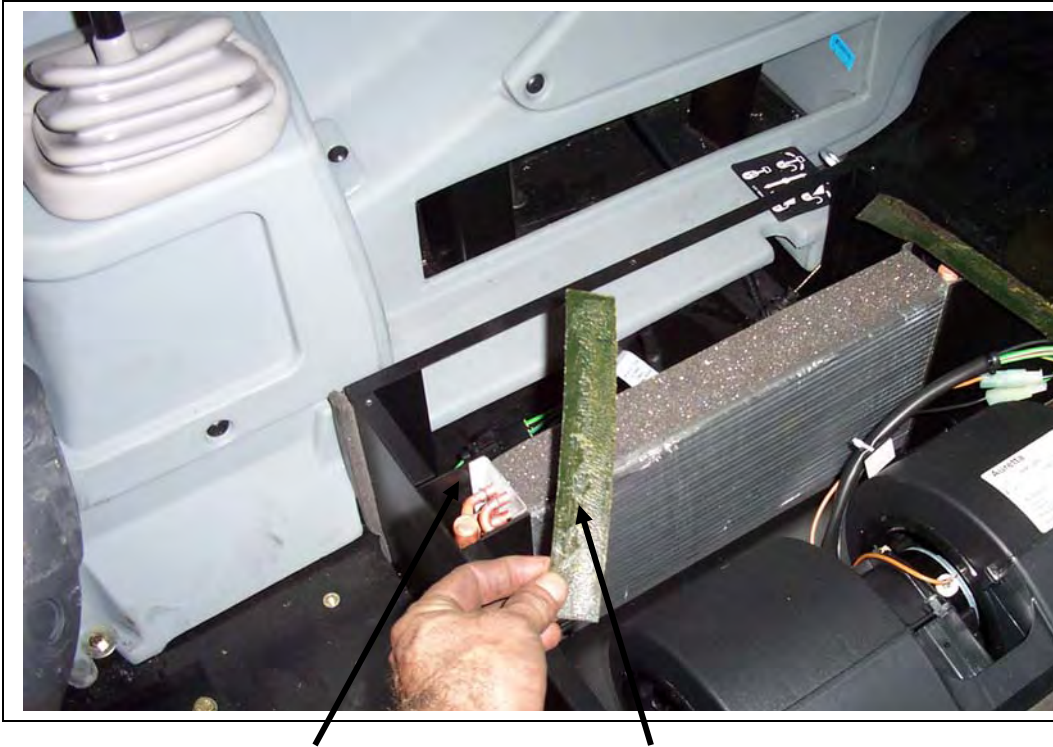
Tar paper gasket was here( same on other end of coil)
