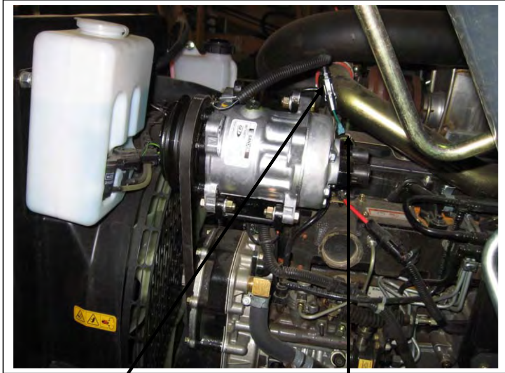
Compressor clutch wire attached to binary switch.
