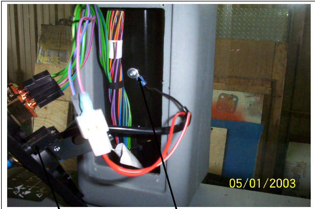
A/C switch mounted on switch panel
