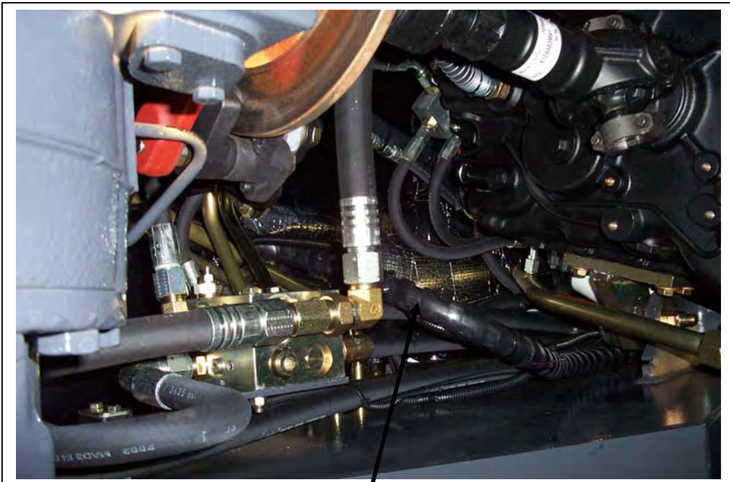
1/2" hose running up and over the rear axle and heading to the right side of the machine to the AC fittings at the heat/AC box.
